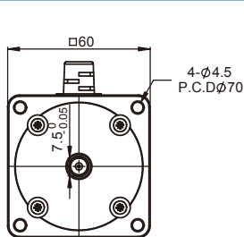
(A-A端子面) Terminal Surface
