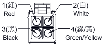
(A-A端子面) Terminal Surface
